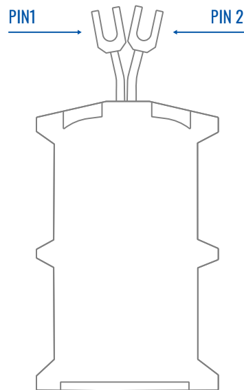
FMC880 socket pinout
